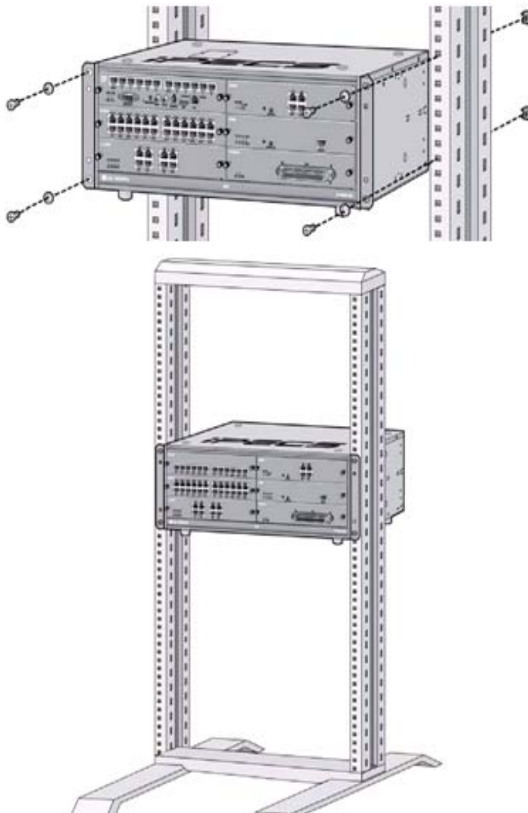
KSU Rack Mounting
