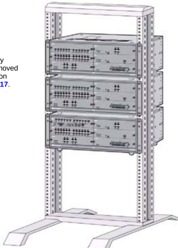
KSU Rack Mounting
